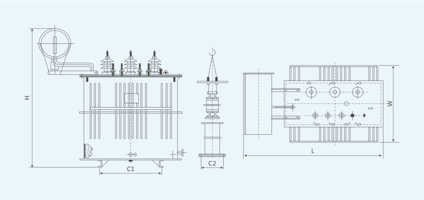
S11-10~2000/10 transformer outline and installation size
