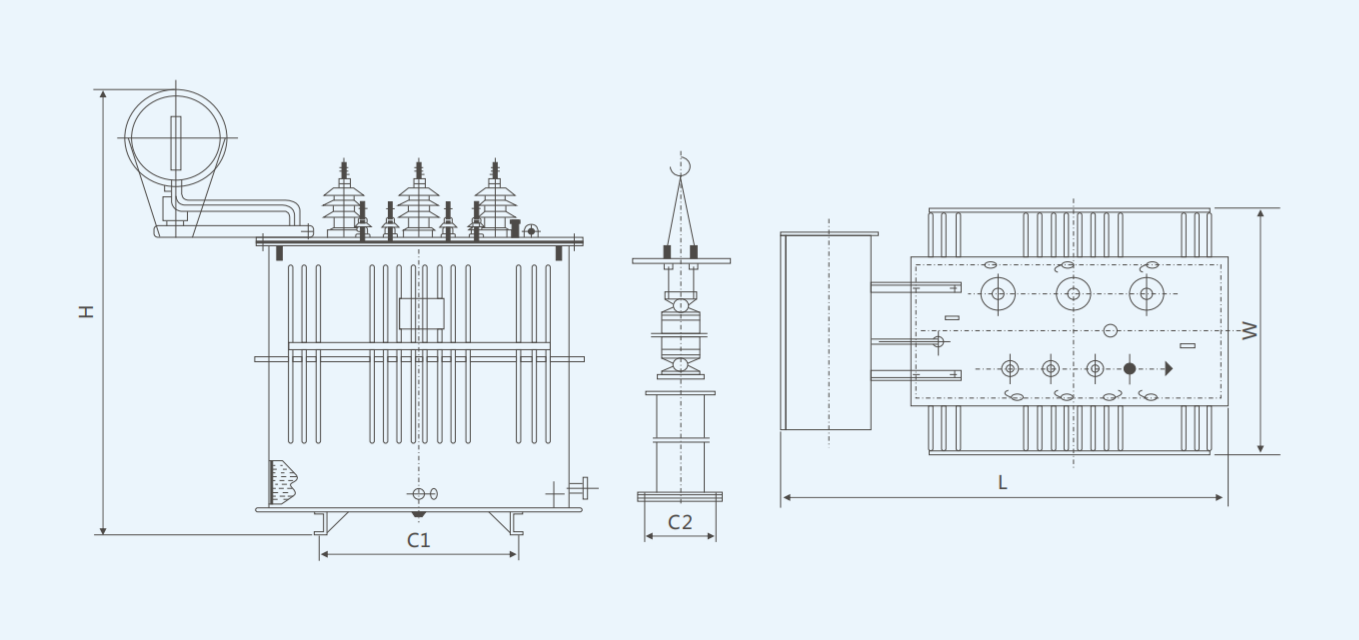
S13-10~2000/10 transformer outline and installation size
