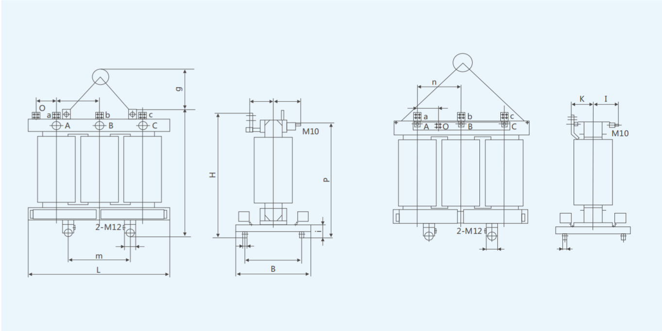
Size drawing of SG(B)10-100~400kVA
